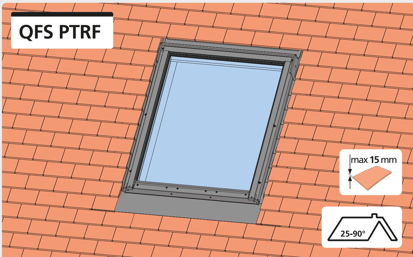
Plain Tile Roof Flashing
